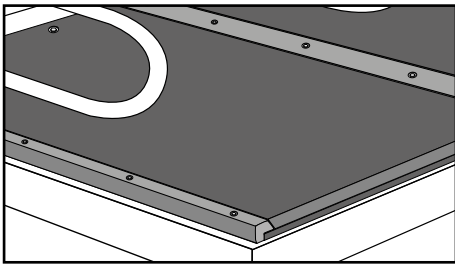
fasten with "end"-profile
